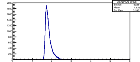
Lossed Energy in ALPIDE circuit at Alpha (d = 19mm)
