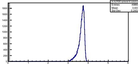
Lossed Energy in ALPIDE epitaxial + substruct at Alpha (d = 19mm)
