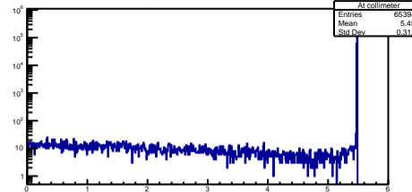
Lossed Energy in collimeter at Alpha (d = 19mm)
